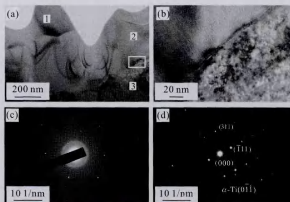
Fig.5 TEM images of interfacial zone of Ti/Cu clad sheet.
