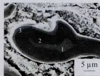
Fig. 3 SEM image of vortex on the explosive welded interface
