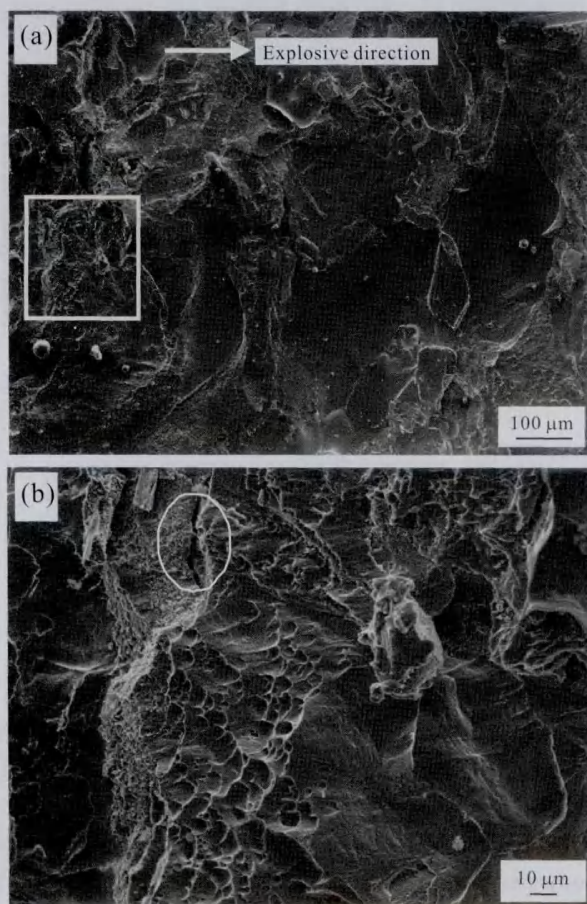
Fig.6 Fracture on the Cu side of explosive welded interface (a) and selected zone magnification (b). The shear force is loaded along the explosive direction
